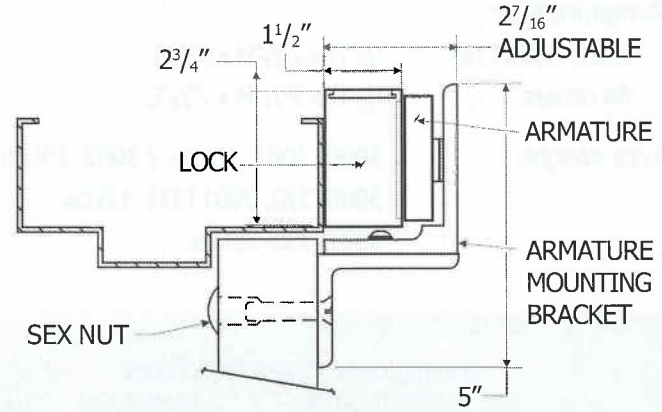
INSWINGING DOOR SIDE VIEW
