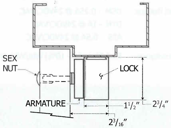
OUTSWINGING DOOR SIDE VIEW
