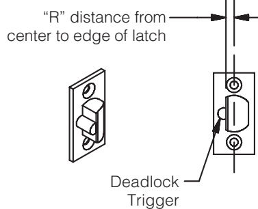
Cylindrical Lock
